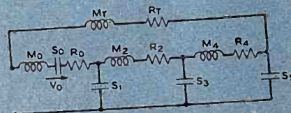
Electrical equivalent of diaphragm type pressure element
